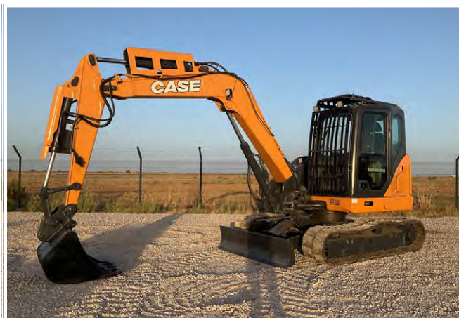
1/2 - 2017 CASE CX80C
